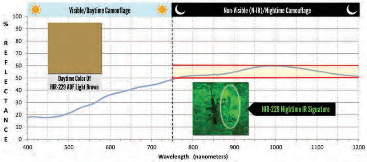
Figure 8. Graph showing visual and N-IR management of HIR-229 ADF Light Brown.
